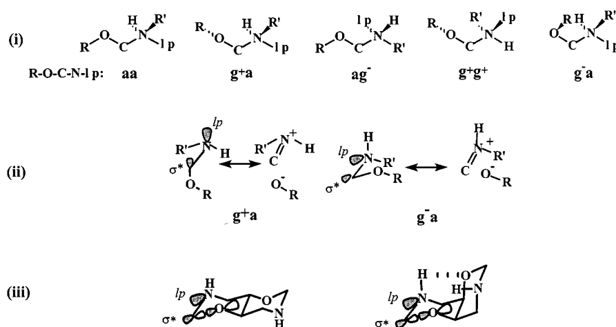
Figure 1. The anomeric effect : (i) in the prototypal R–O–C–N–R' moiety (uniquely defined by the N lone pair and OR termini); (ii) with MO visualization of its geometrical consequences; (iii) in the 1,3-oxazane system of trans - and cis -DODAD
