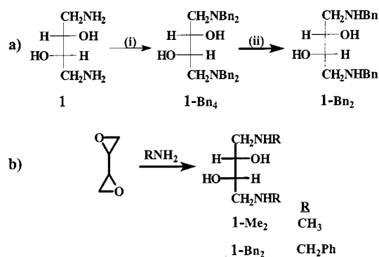
Scheme 3. Preparation of N,N' -dialkyl threo -1,4-diamino-2,3-butanediols: (a) benzylation of 1 : (i) benzyl bromide/ \text{K}_2\text{CO}_3 aq.; (ii) \text{H}_2 , Pd/C, HCl. (b) from threo -1,2;3,4-diepoxybutane
