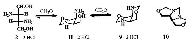
Scheme 6. Reaction of D -threo-2,3-diamino-1,4-butanediol ( 2 ) with formaldehyde
